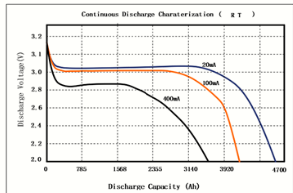
Different Temp. Discharge Curve at 20mA
